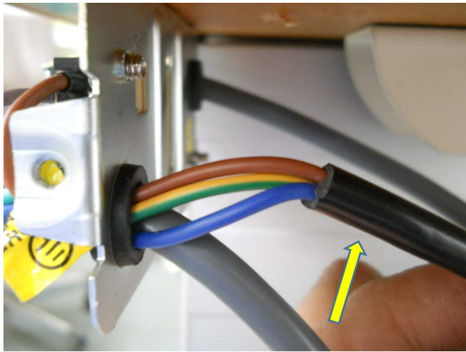
CS-2 main electric cable merge to main switch
