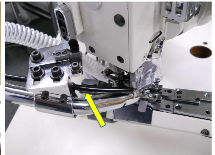
Suction device ⑦
