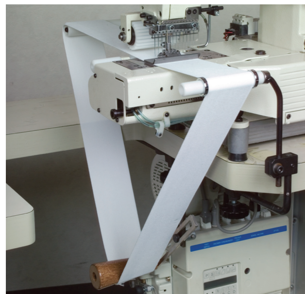
■ RT-1 ゴム張り装置 (手動式) DX, FX (PSF, PMD, PLは除く), RX (RX-P, PLKのみ) RT-1 Elastic expander device ( manual operation ) DX, FX (except for PSF, PMD, PL), RX ( Only for RX-P, PLK ) RT-1 EXPANDIDOR DE ELASTICO DX, FX, RX 松紧带撑开装置 (DX,FX, 除PSF, PMD, PL, RX-P, PLK)
