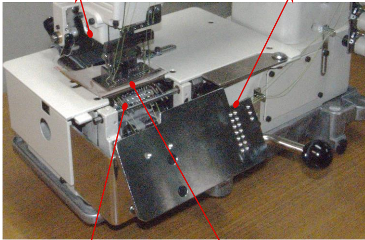
Metal Gear Puller with double lower puller
