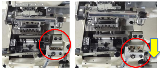
skip stitch device OFF skip stitch device ON
