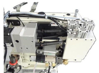
Rear puller controlled by pulse motor
