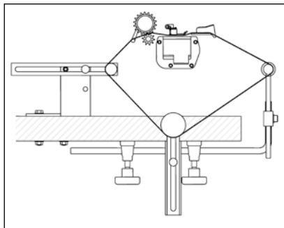
■ RT-1 ゴム張り装置 (手動式) DX, FX(PSF, PMD, PLは除く), RX (RX-P, PLKのみ) RT-1 Elastic expander device ( manual operation ) DX, FX (except for PSF, PMD, PL), RX ( Only for RX-P,PLK) RT-1 EXPANDIDOR DE ELASTICO DX, FX, RX 松紧带撑开装置 (DX,FX, 除PSF, PMD, PL, RX-P, PLK)
