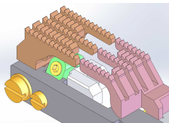
Differential feed mechanism prevents puckering
