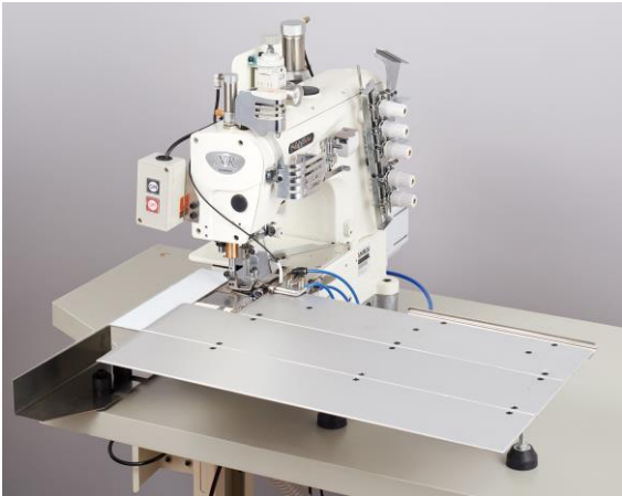
ABH-2R Semi-automatic hemming device for T-shirts sleeves.
