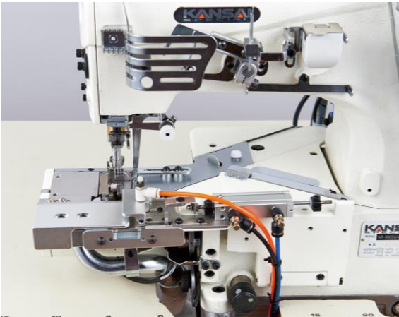
ABH-1M Pneumatic hemming guide with knee switch. Hemming is folded by air-blower without handling.
