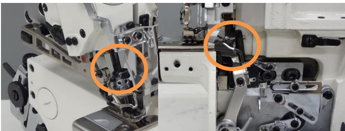
DLC needle bar and upper looper holder for oil leakage prevention, last in high speed operation
