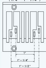
DLR1508P (1/4" - 1-1/4")
