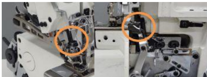
DLC needle bar and upper looper holder for oil leakage prevention, last in high speed operation
