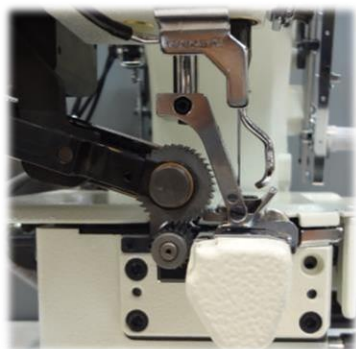
Steel made top & bottom puller
