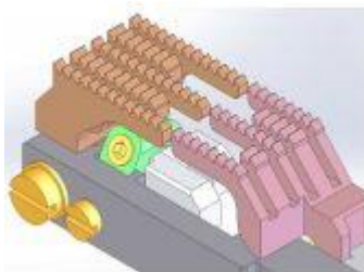
Differential feed mechanism prevents puckering
