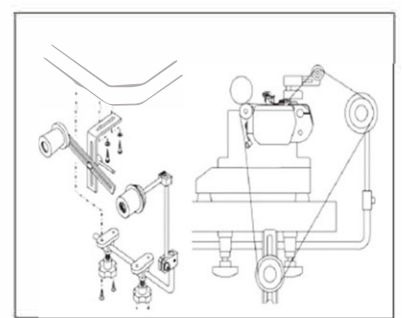
■ RT-1A ゴム張り装置 (エア式) for NR-PHK Elastic expander for NR-PHK
